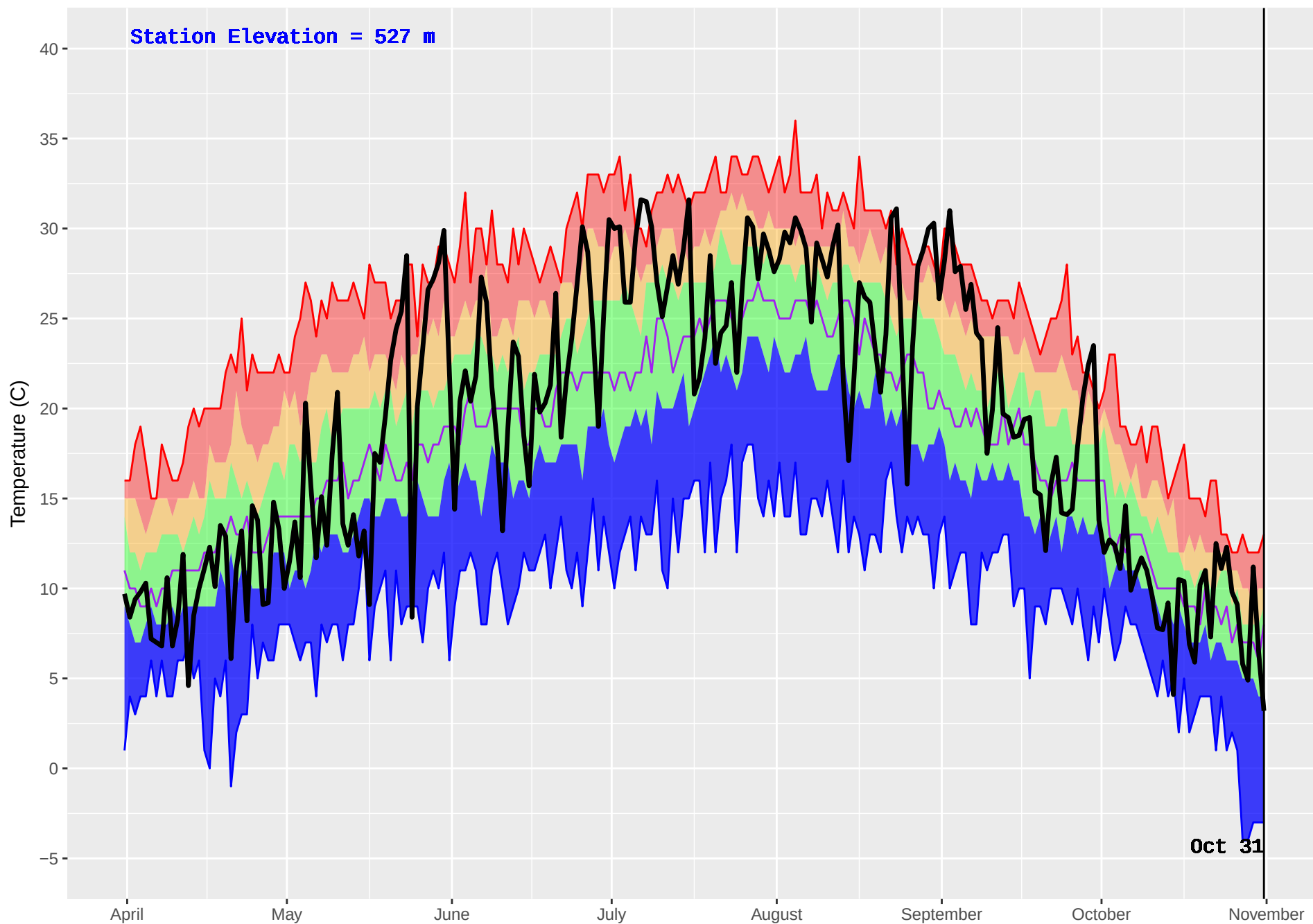
SALMON ARM (346) : Historical (1976–2016) and Current (2017) Noon Temperature
