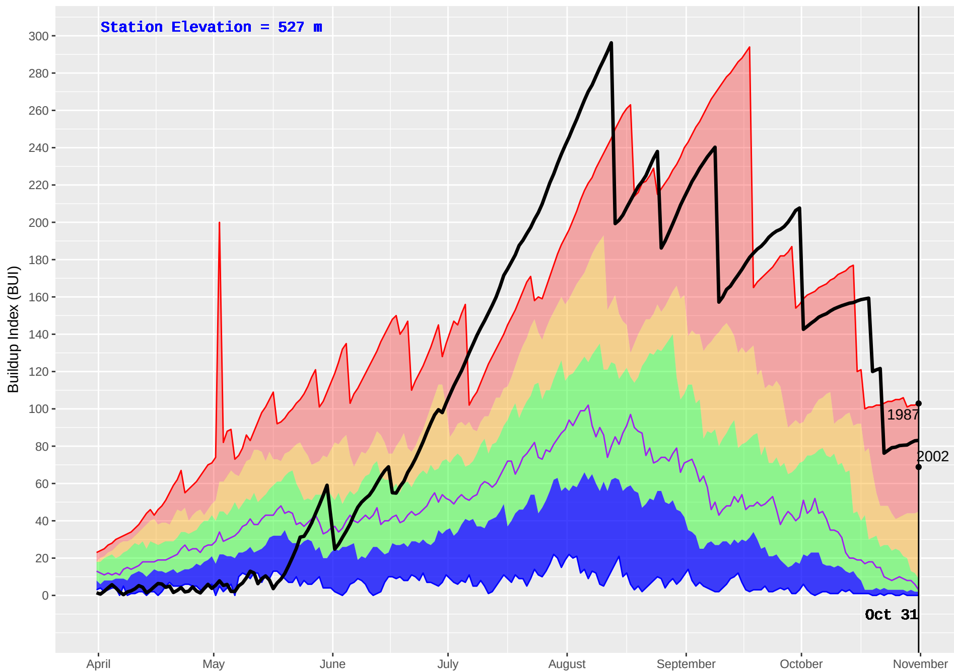
SALMON ARM (346) : Historical (1976–2016) and Current (2017) Noon Buildup Index (BUI)
