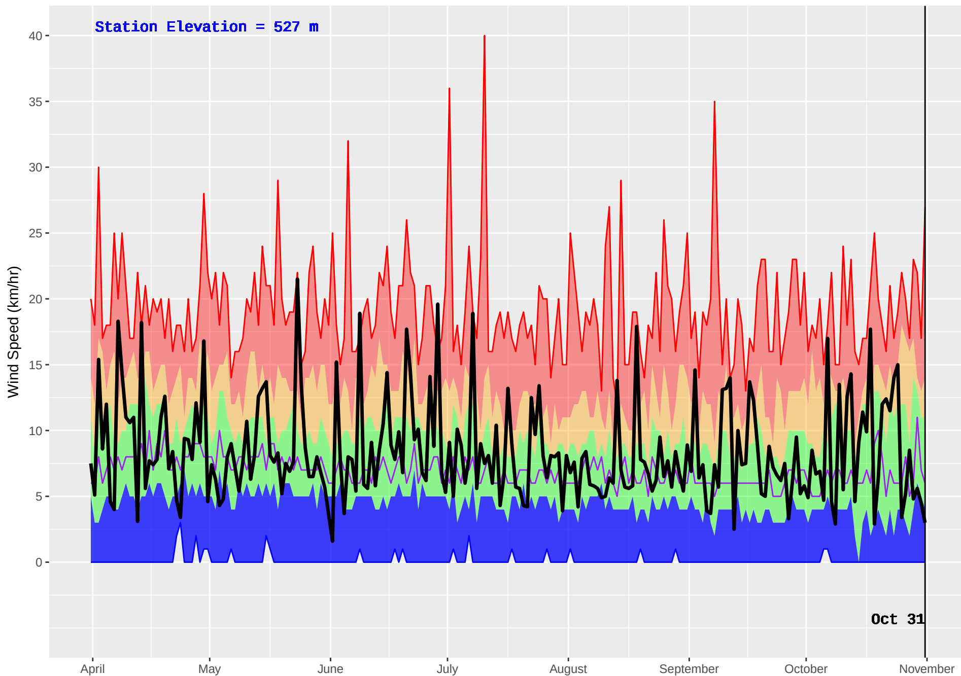
SALMON ARM (346) : Historical (1976–2016) and Current (2017) Noon Wind Speed
